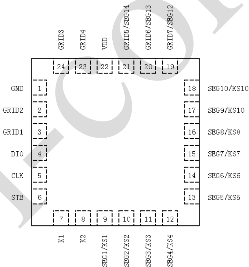
QFN24
