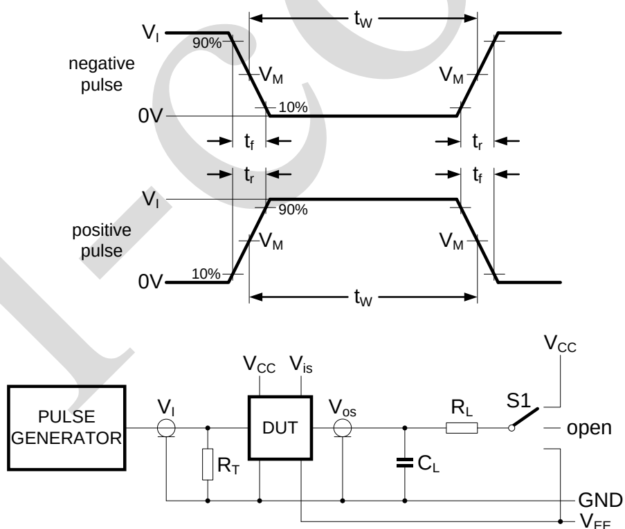
Figure 11. Test circuit for measuring switching times
