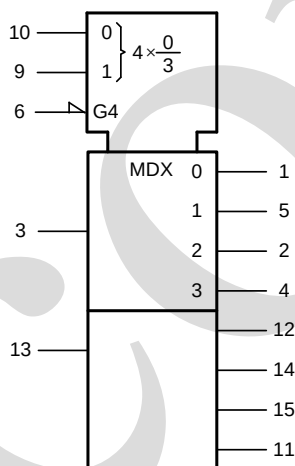
Figure 2. IEC logic symbol
