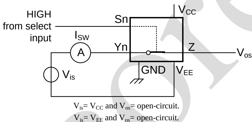
Figure 8. Test circuit for measuring ON-state current
