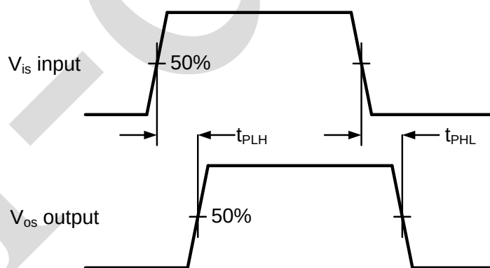
Figure 9. Input ( V_{is} ) to output ( V_{os} ) propagation delays
