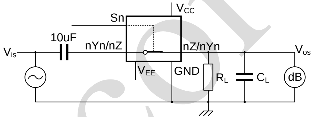
Figure 12. Test circuit for measuring sine-wave distortion
