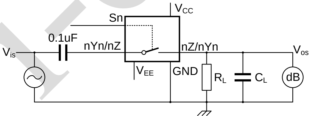
Figure 12. Test circuit for measuring sine-wave distortion
