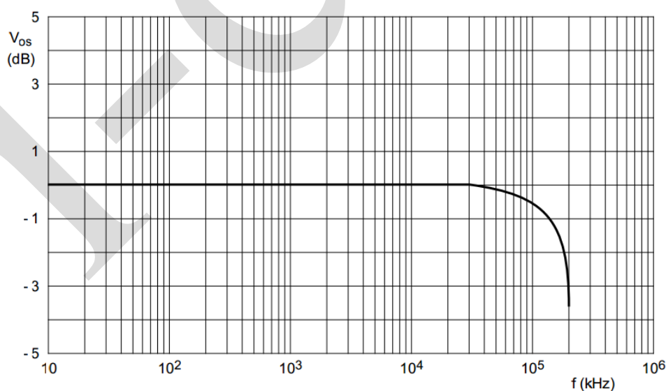
b. Typical frequency response
