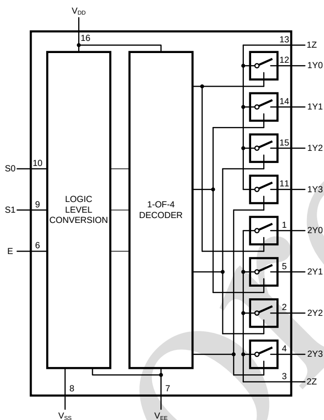
Figure 4. Functional diagram
