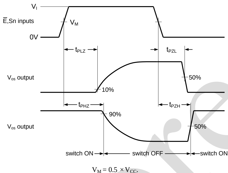
Figure 10. Turn-on and turn-off times
