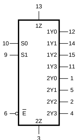
Figure 1. Logic symbol
