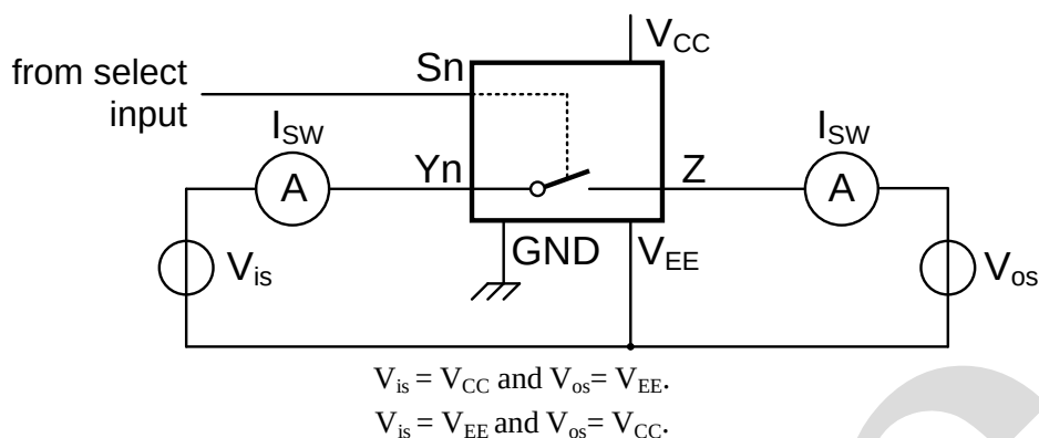
Figure 7. Test circuit for measuring OFF-state current
